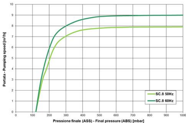
POMPA / PUMP
